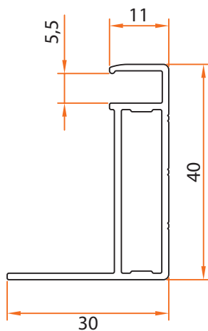
Code: 1449 0,409 kg/m
