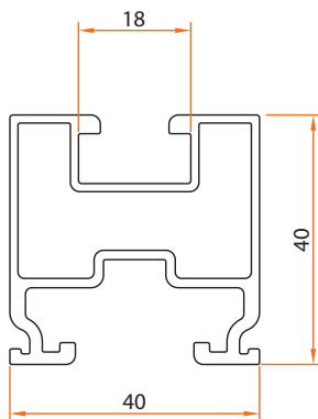
Code: 1424 0,914 kg/m
