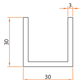
Code: 1437 0,683 kg/m
