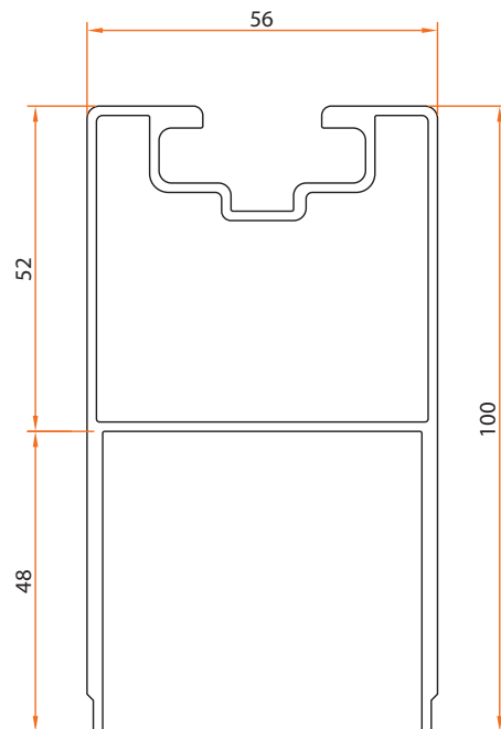
Code: 1434 1,735 kg/m
