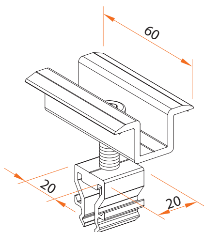
Code: AK-5410
