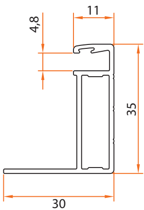
Code: 1448 0,385 kg/m
