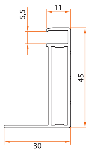
Code: 1450 0,444 kg/m
