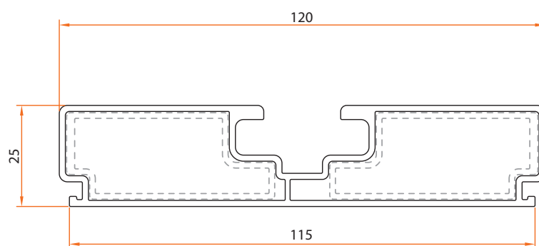
Code: 1412 1,455 kg/m
