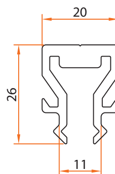
Code: 1422 0,585 kg/m
