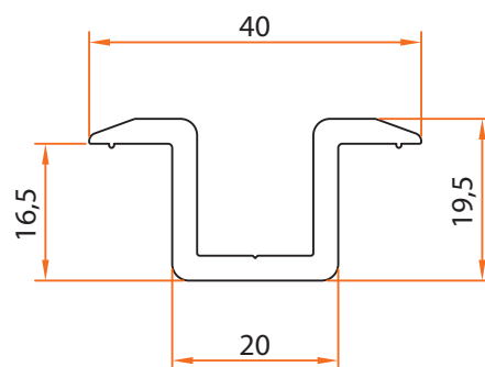
Code: 1420 0,555 kg/m
