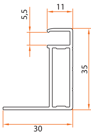
Code: 1446 0,374 kg/m
