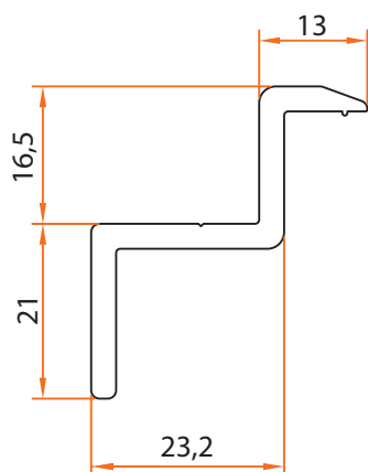
Code: 1419 0,530 kg/m
