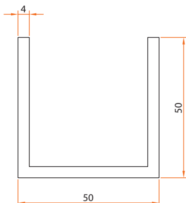
Code: 1435 1,539 kg/m
