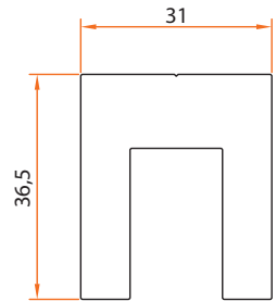
Code: 1438 2,070 kg/m
