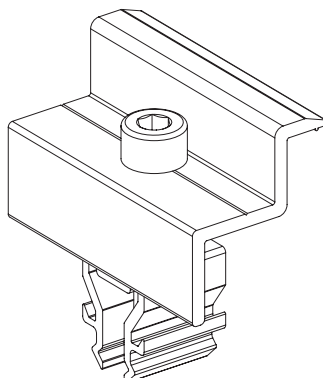
Code: AK-5411
