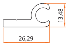
Code: 1416 0,373 kg/m
