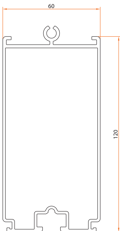
Code: 1411 1,964 kg/m
