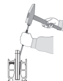
AK-5299 Wedge Fixing Tool
