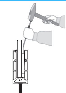
AK-5299 Wedge Fixing Tool
